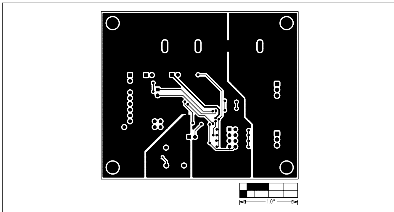
Figure 6. MAX6616 EV Kit PC Board Layout—Solder Side
